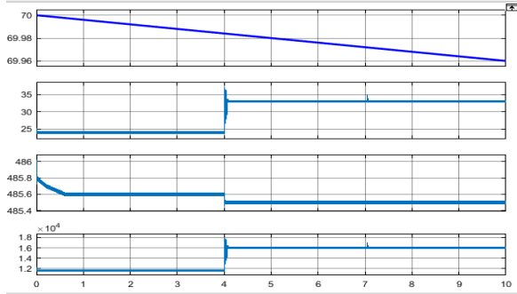
Fig shows EV2 state of charge, EV2 battery current, EV2 battery voltage, EV2 battery power
