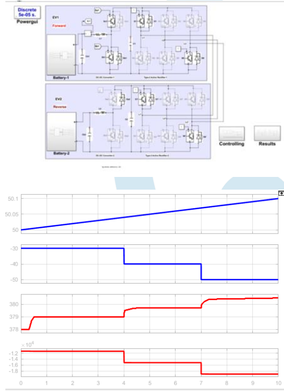
Fig shows EV1 state of charge, EV1 battery current, EV1 battery voltage, EV1 battery power
