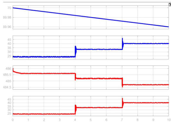
Fig shows EV2 state of charge, EV2 battery current, EV2 battery voltage, EV2 battery power
