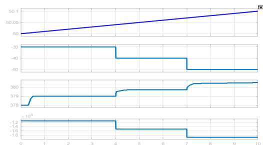
Fig shows EV1 state of charge, EV1 battery current, EV1 battery voltage, EV1 battery power
